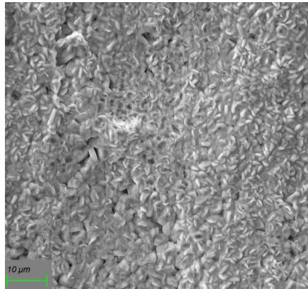
SURFACOTE 780, 1000x magnification
